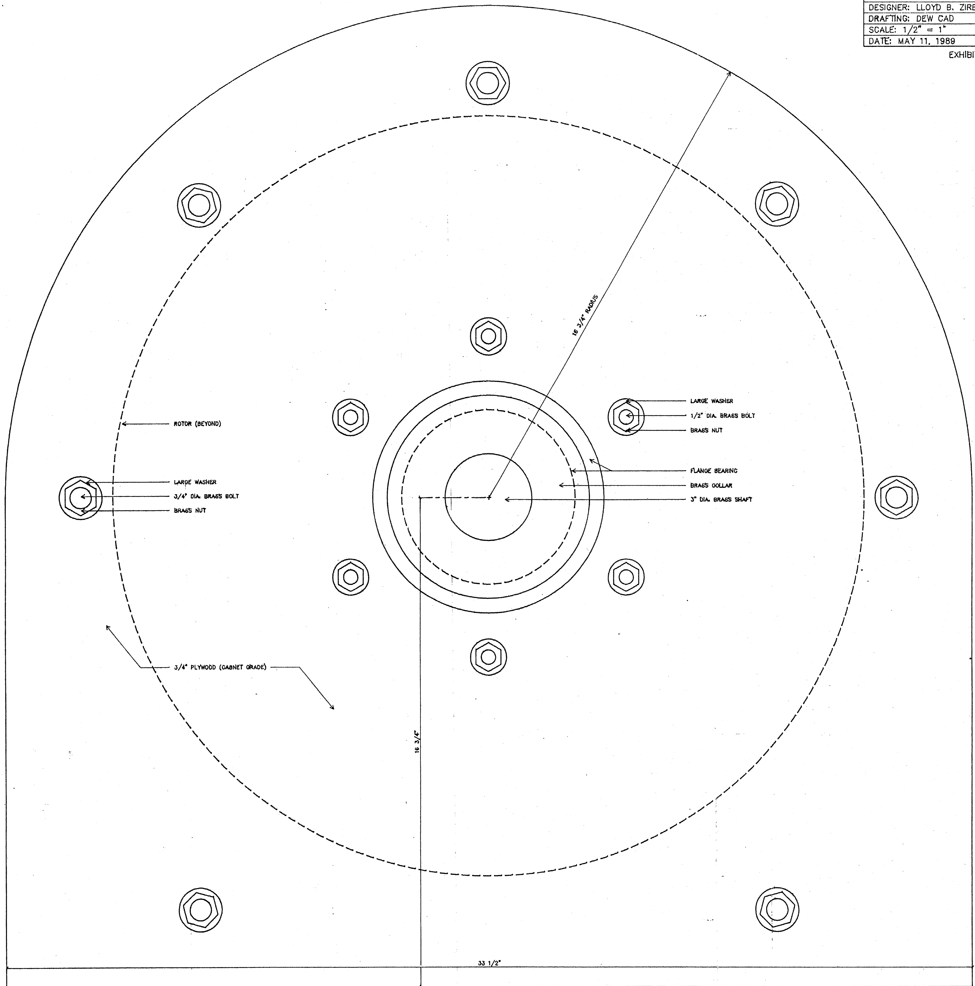
BACK VIEW
