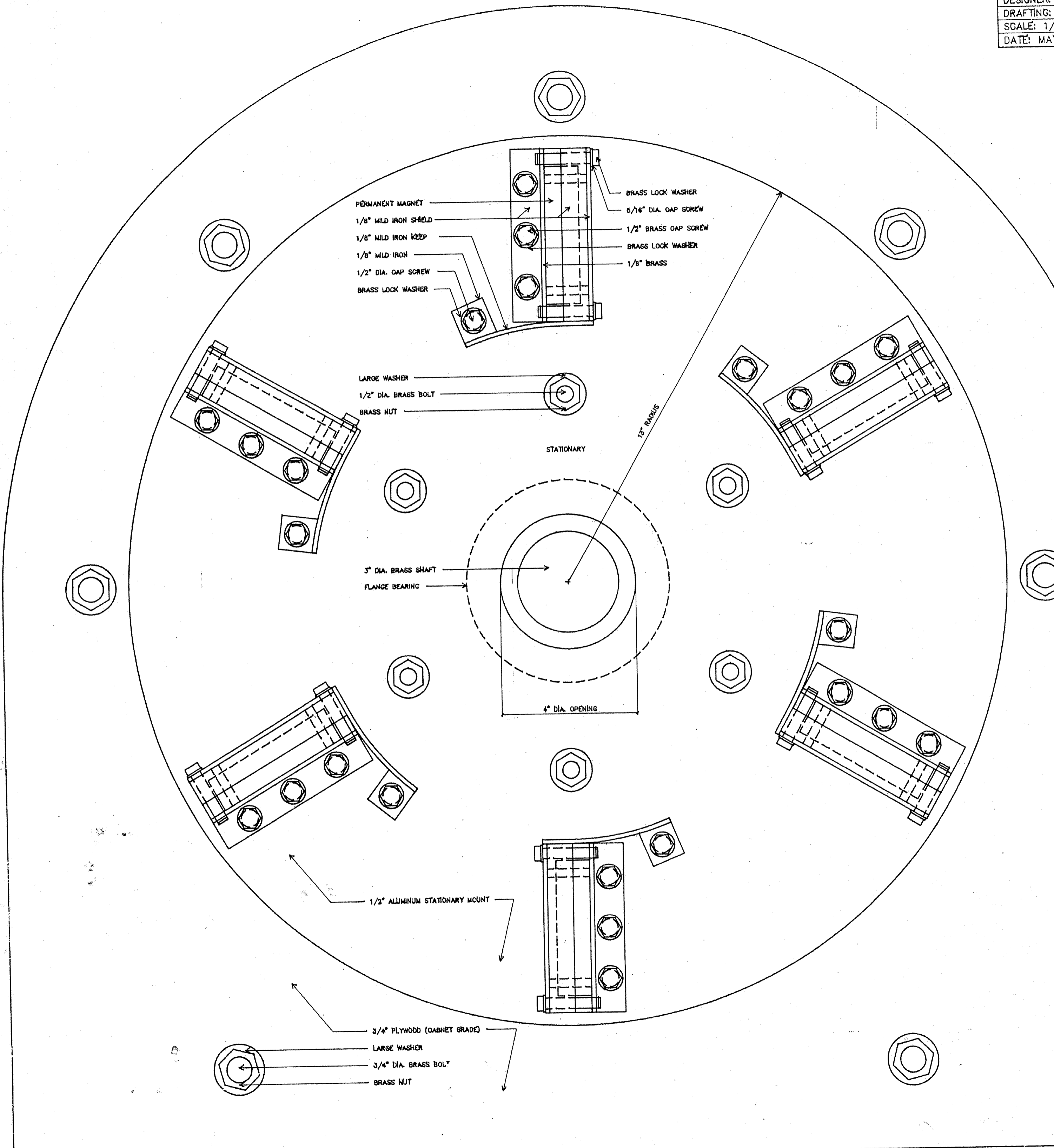
STATIONARY MOUNT (LOOKING TOWARDS BACK)
